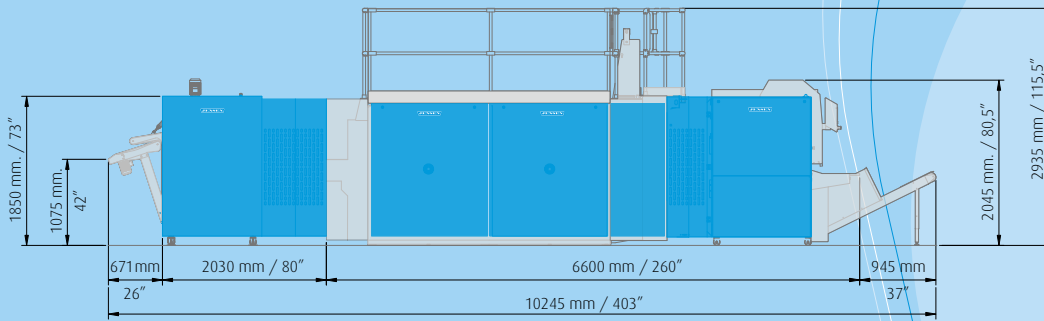
Side view Jenfeed Express in a JENSEN Express line
